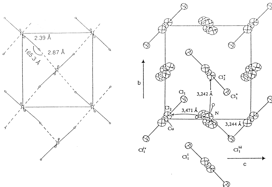
Fig. 3. Layer salts showing cooperative Jahn–Teller distortions: left hand side (\text{H}_3\text{N}(\text{CH}_2)_3\text{NH}_3) \text{CrCl}_4 [12]; right hand side (\text{H}_3\text{N}(\text{CH}_2)_4\text{NH}_3) \text{CuCl}_4 [8].
