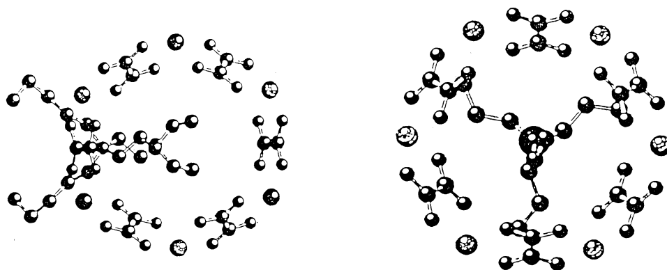
Fig. 5. Arrangement of the organic cations relative to the complex anion layers in N(n-C_nH_{2n+1})_4 - MM'(C_2O_4)_3 : left hand side, n = 5 ; right hand side, n = 3 .
