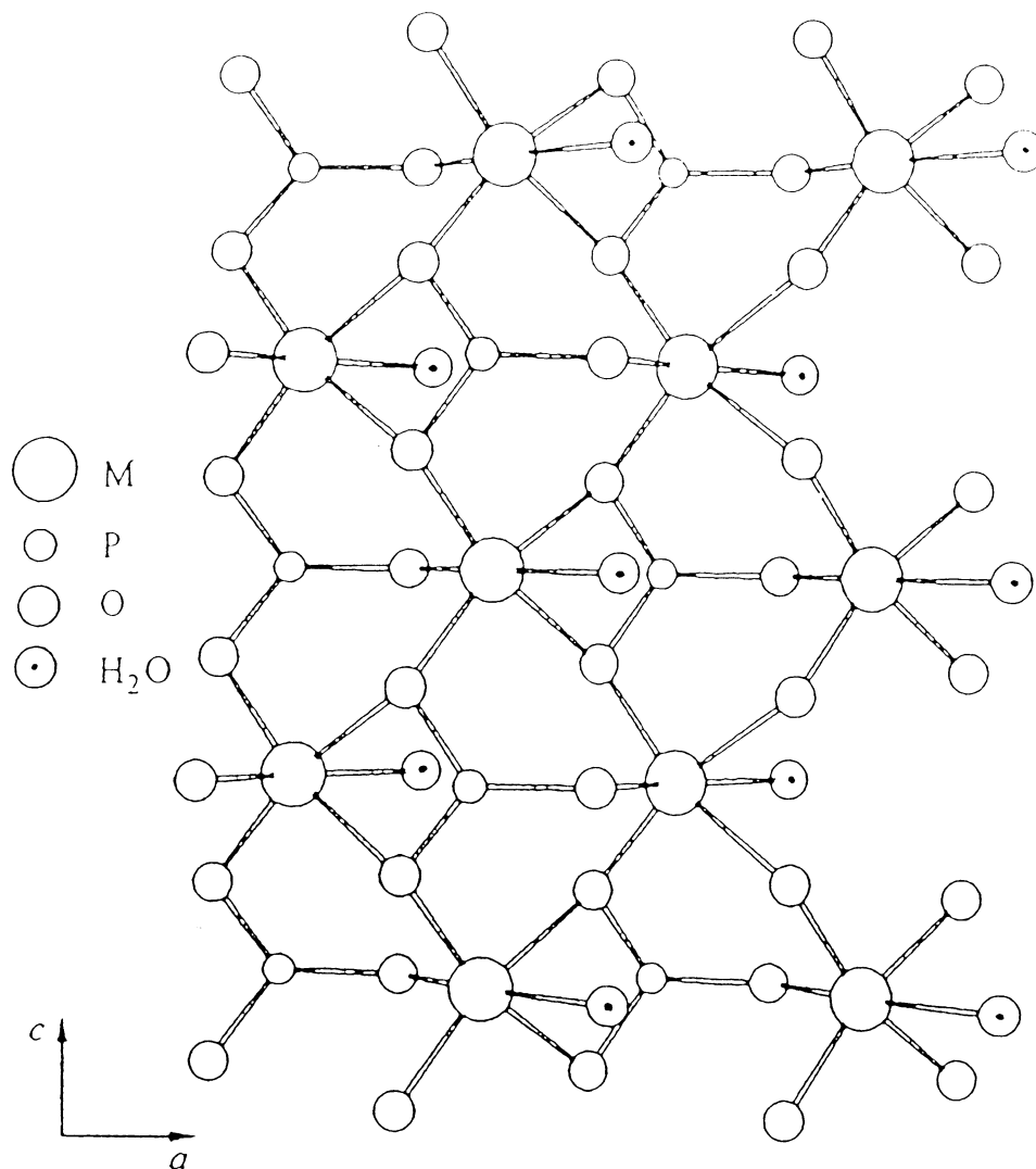
Fig. 4. The 4-connected net in the basal plane of (\text{RPO}_3)_n\text{M} \cdot n\text{H}_2\text{O} [13].
